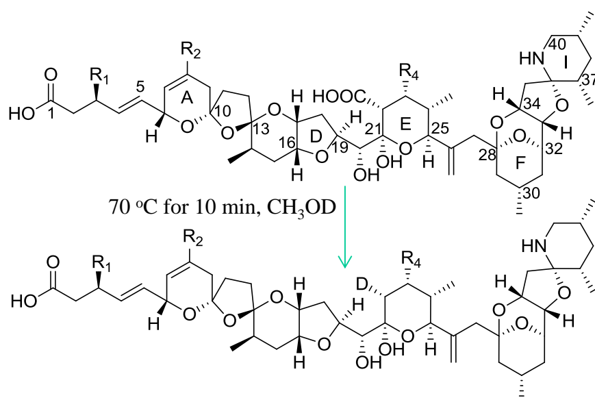
Figure S7. At higher temperatures (or during storage) and in the presence of deuterated methanol, C-22 carboxylated analogues will decarboxylate and incorporation of deuterium (D) will occur.
