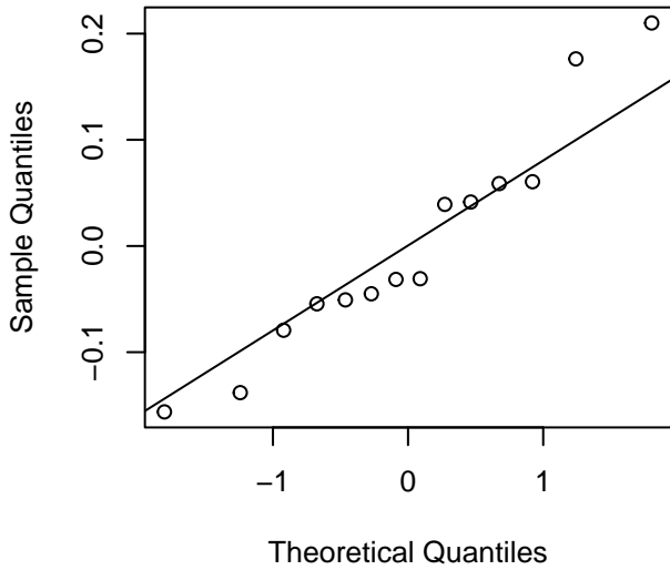
Normality Residuals
